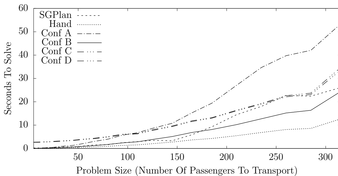
Figure 6.20: Planning times in ZENO domain, without FF
