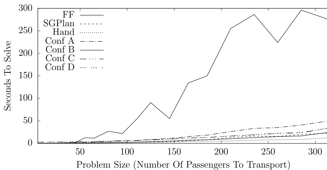
Figure 6.19: Average planning times in ZENO domain
