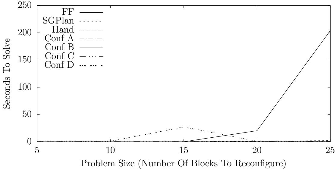
Figure 6.15: Average planning times in BLOCKS-WORLD domain
