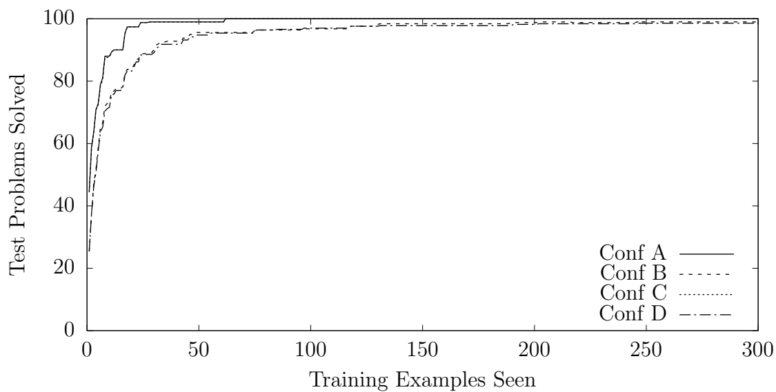
Figure 6.11: Learning rate in LOGISTICS domain
