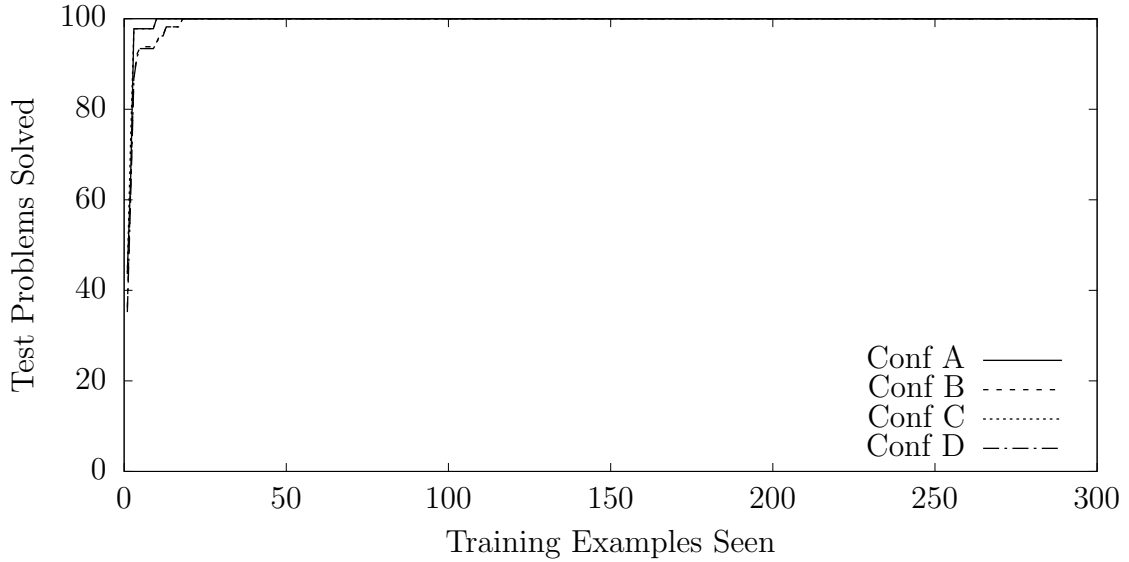
Figure 6.12: Learning rate in ZENO domain
