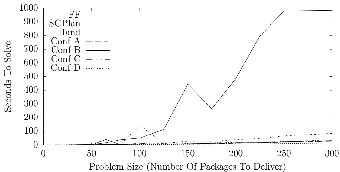
Figure 6.17: Average planning times in LOGISTICS domain
