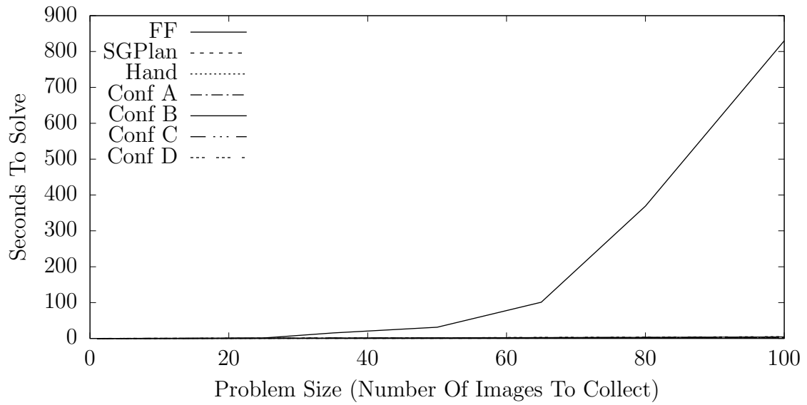
Figure 6.21: Average planning times in SATELLITE domain
