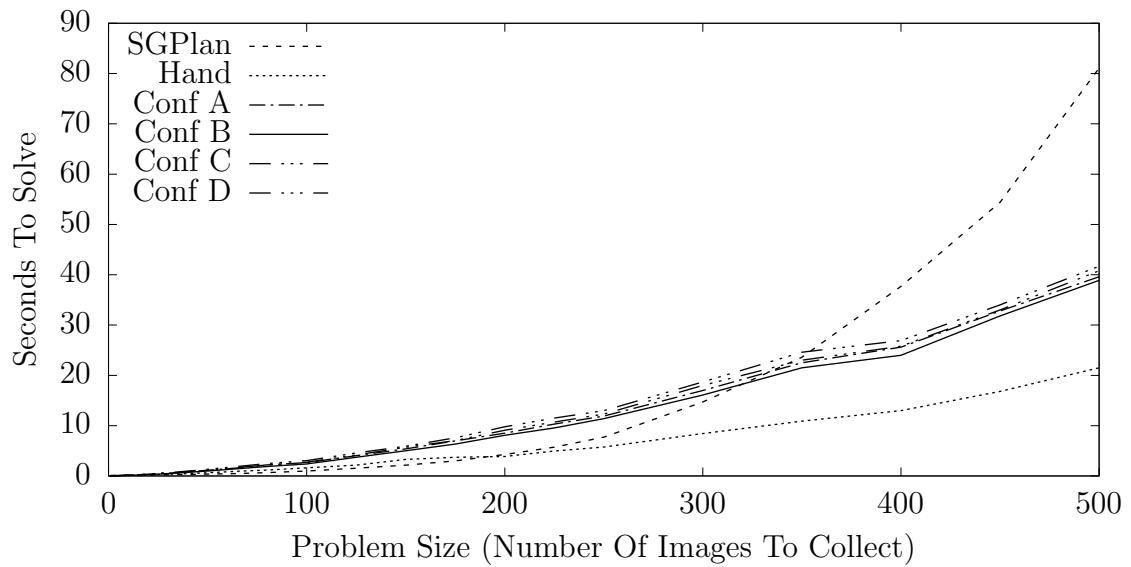
Figure 6.22: Planning times in SATELLITE domain, without FF
