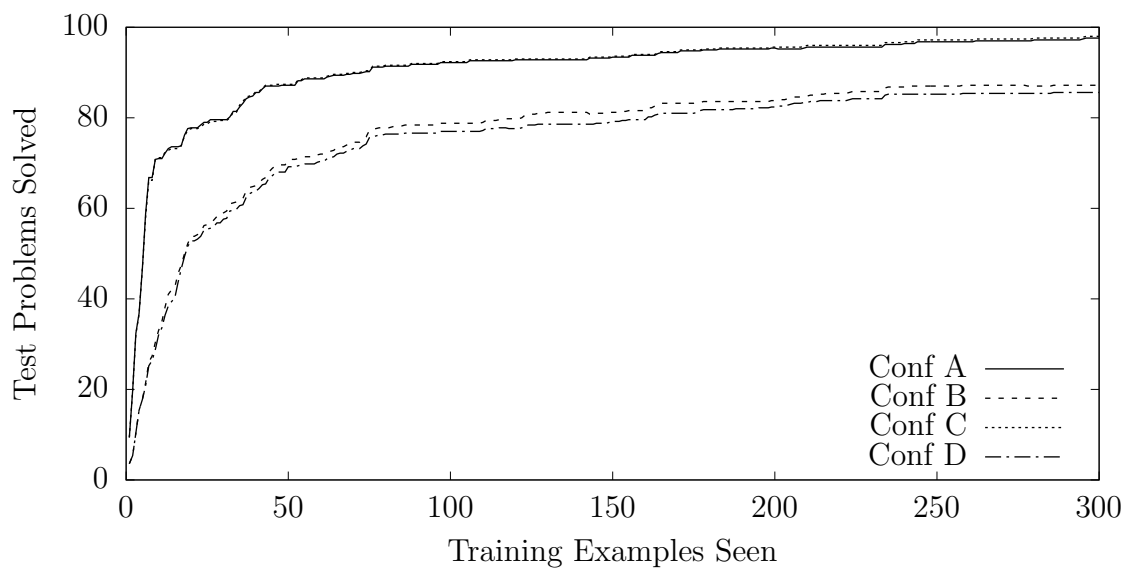
Figure 6.14: Learning rate in ROVERS domain
