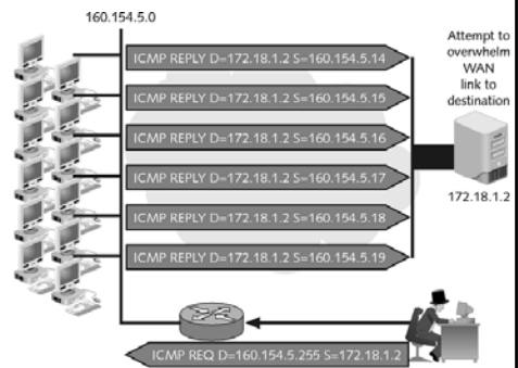
Figure 3-4 Smurf attack
